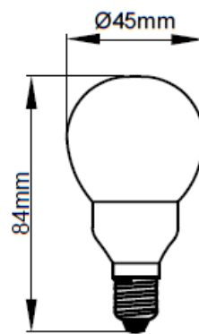
KCF07GLF/E14
