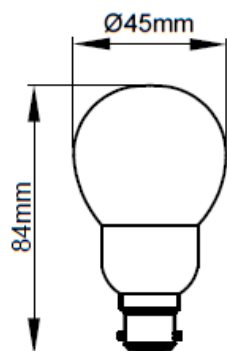
KCF07GLF/B22
