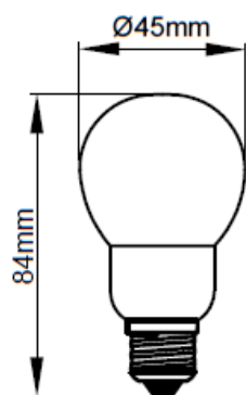
KCF07GLF/E27
